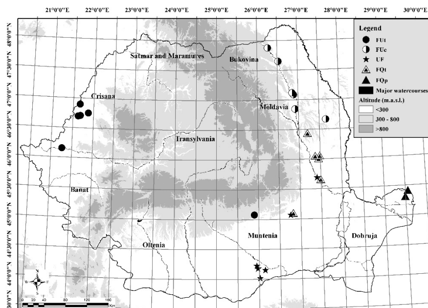
Fig. 2. The synchronological map of the floodplain forests in the plain areas of Romania: Fraxino pan-nonicae-Ulmetum glabrae typicum (FUt), Fraxino pan-nonicae-Ulmetum glabrae euonymetosum nanae (FUE), Ulmo campestris-Fraxinetum holotrichae (UF), Fraxino pallisae-Quercetum pedunculiflorae typicum (FQt), Fraxino pallisae-Quercetum pedunculiflorae periplocetosum graecae (FQp).
